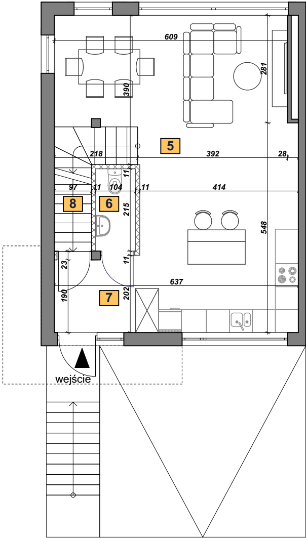
parter
